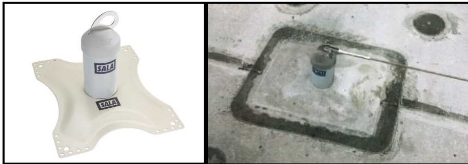
Roof-mounted Evolution End Post (New and Installed)
